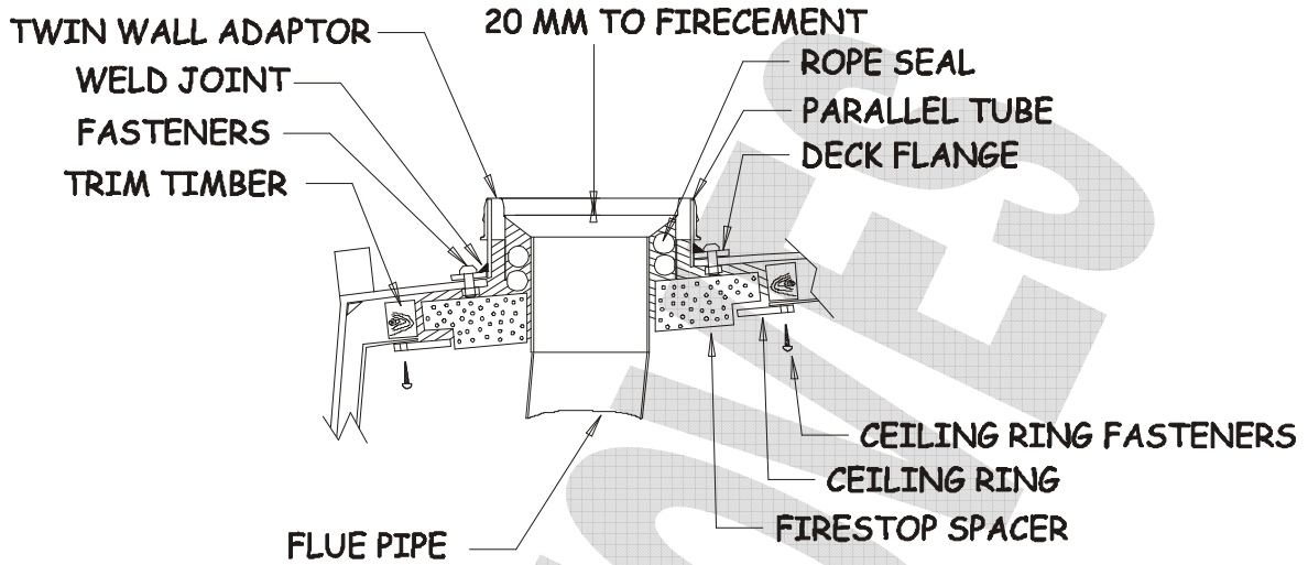
FIG 1 ASSEMBLY DETAILS
